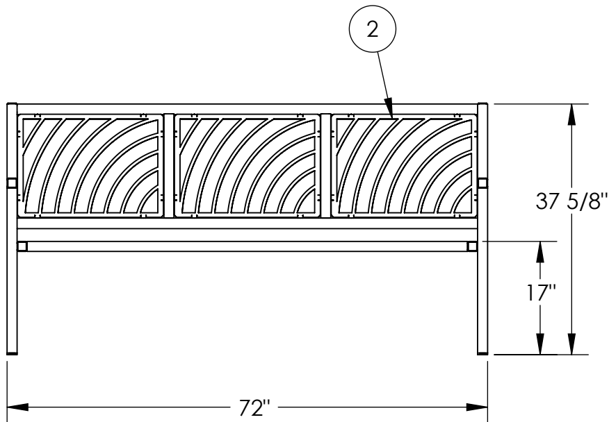
FRONT VIEW
