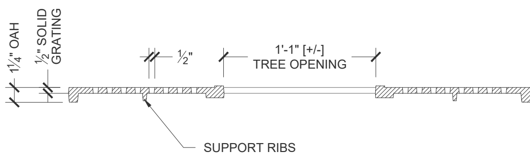
Cross Section Scale: 1 1/2" = 1' 0"
