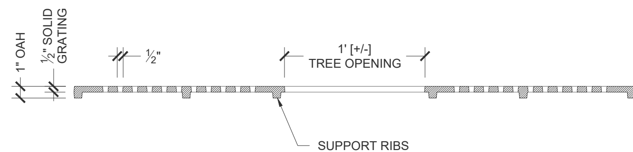
Cross Section Scale: 1 1/2" = 1' 0"
