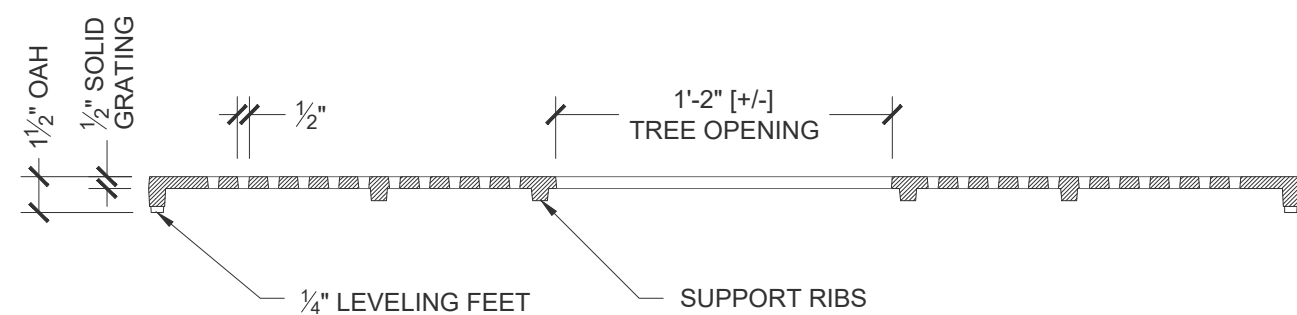
Cross Section Scale: 1 1/2" = 1' 0"
