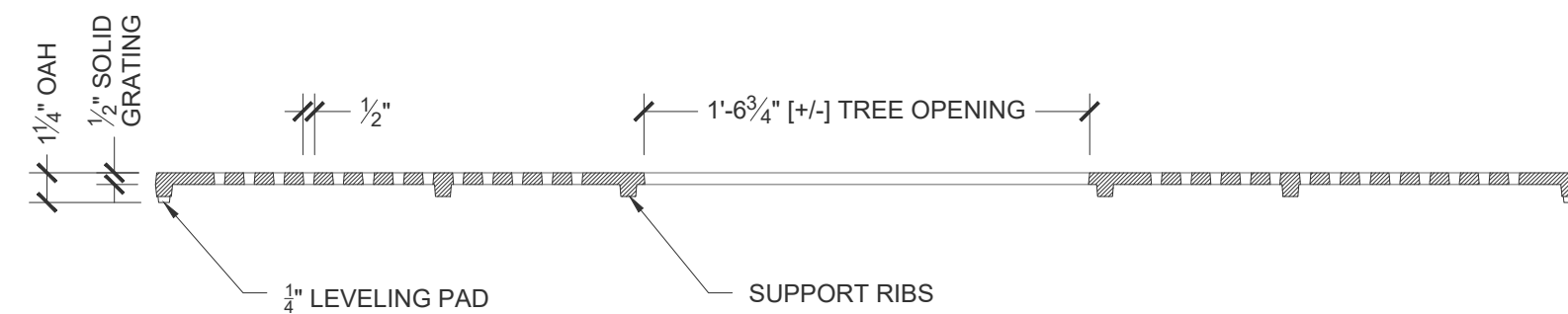
Cross Section Scale: 1 1/2" = 1' 0"
