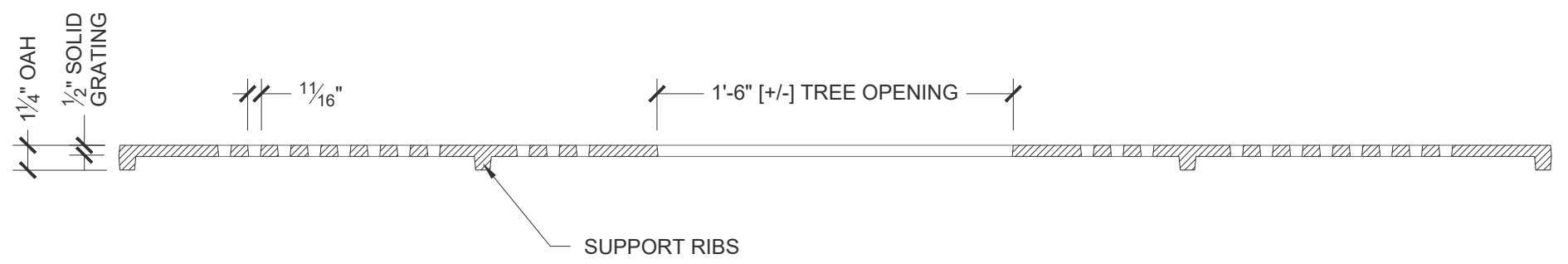
Cross Section Scale: 1 1/2" = 1' 0"
