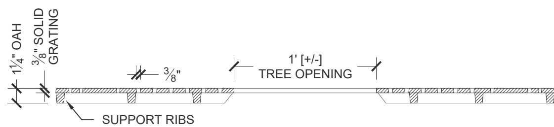
Cross Section Scale: 1 1/2" = 1' 0"
