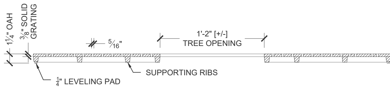
Cross Section Scale: 1 1/2" = 1' 0"
