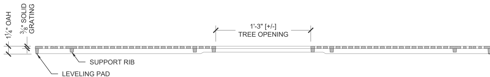
Cross Section Scale: 1 1/2" = 1' 0"
