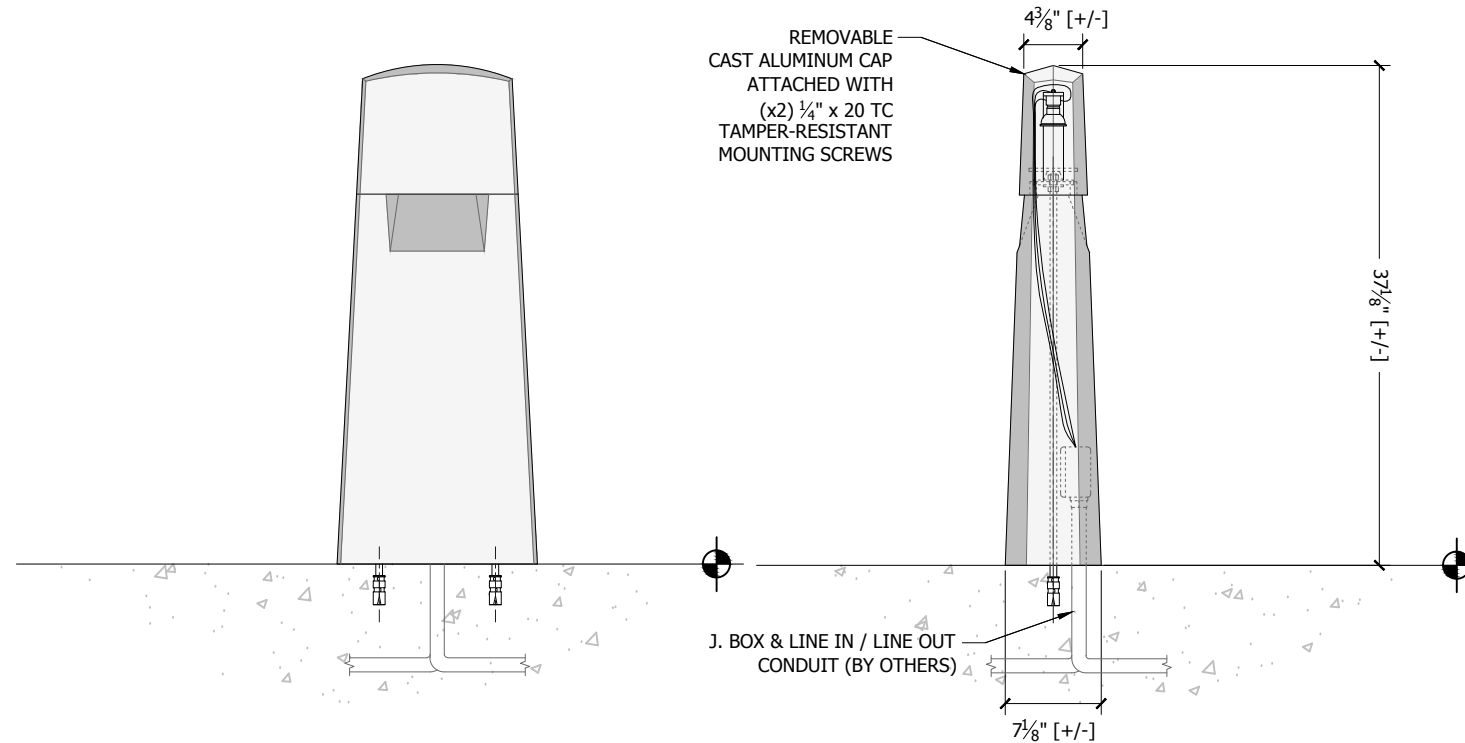
Front Elevation
